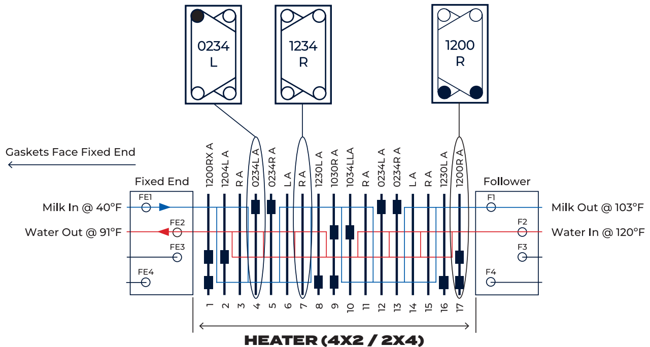
Figure 9 Heater Section
